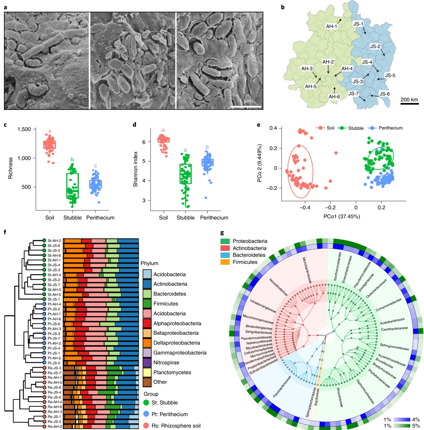
Fig. 1 | Assessment of perithecium-associated bacterial communities. a , Scanning electron microscopy observation of bacteria on perithecia collected from the field. The experiment was repeated three times with similar results. b , Locations of 13 sampling sites located in two Chinese provinces. AH, Anhui Province; JS, Jiangsu Province. c–d , Richness ( c ) and Shannon ( d ) index of the bacterial communities from perithecia, rice stubbles and soil. Different letters indicate significantly different groups ( P < 0.001 , ANOVA, Tukey's HSD). The horizontal lines within boxes represent medians. The tops and bottoms of boxes represent the 75th and 25th percentiles, respectively. The upper and lower whiskers extend to data no more than 1.5 \times the interquartile range from the upper edge and lower edge of the box, respectively. e , Principal coordinates analysis based on Bray-Curtis distance showing that the microbiota of perithecia is distinct from that of soil and rice stubbles ( P = 0.001 , PERMANOVA with ADONIS test). f , Stacked bar plot combined with Bray-Curtis distance-based dendrogram showing the averaged bacterial community composition for each compartment at each sampling site. The stacked bar plot includes the phylum and proteobacterial class levels as indicated. g , The core microbiome of perithecium-associated bacteria. The inner ring represents the OTUs that were reproducibly detected in the perithecia and infected rice stubbles with relative abundance greater than 0.1%. The relative abundances of distinct perithecium and stubble OTUs are shown as blue (perithecium) and green (stubble) heatmaps. Replicates for each compartment, n = 65 biologically independent samples.
